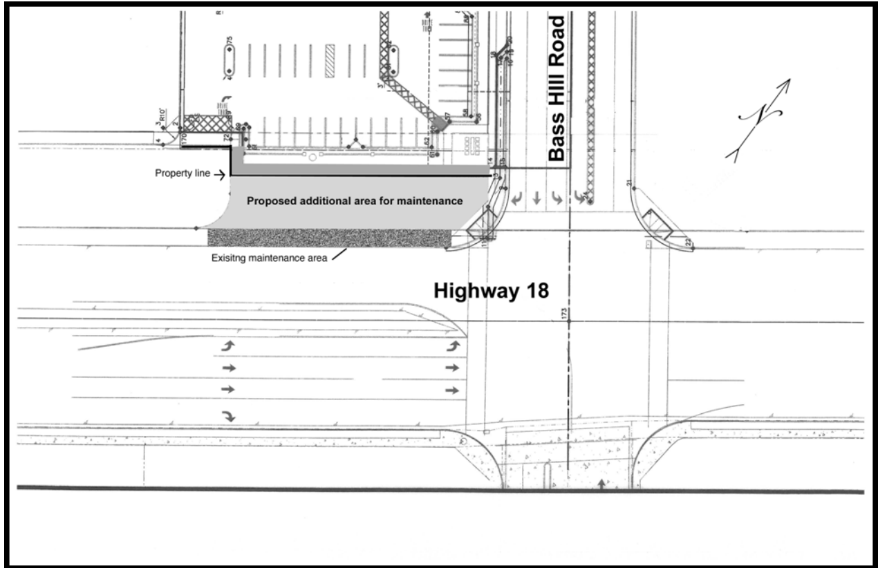
AVLLAD #1, L-23- Detail for northwest corner of Highway 18 and Bass Hill Road Additional Maintenance Area (Added by Council Action 6/12/12)
