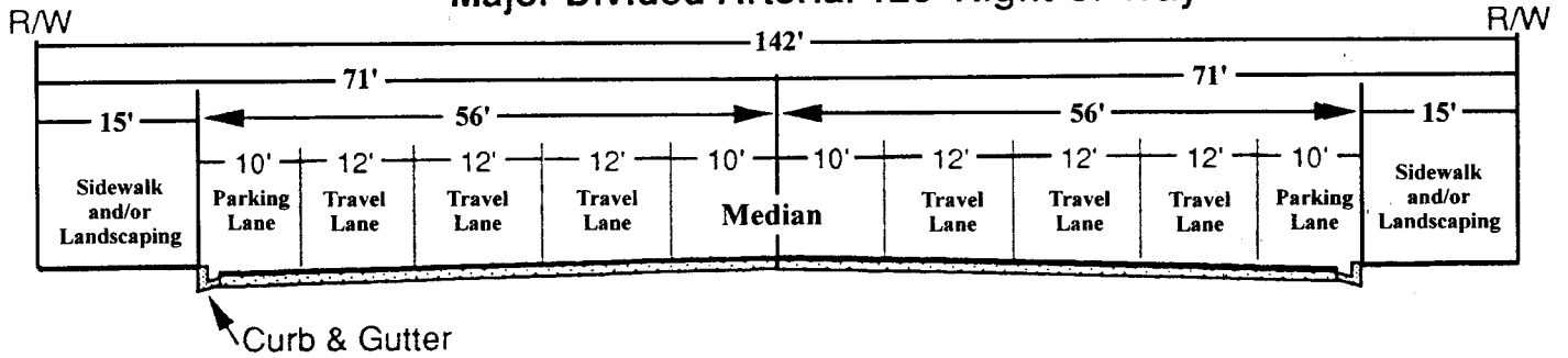
Alternate Major Divided Arterial 142' Right-of-Way
