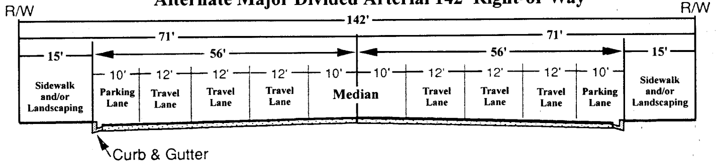
Alternate Major Divided Arterial 142' Right-of-Way (Modified Section)
