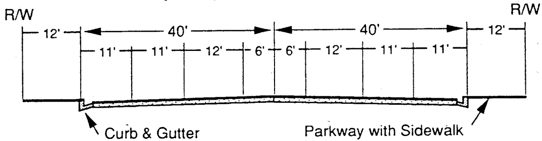
Major Highway 104' Right-of-Way (Modified Section)
