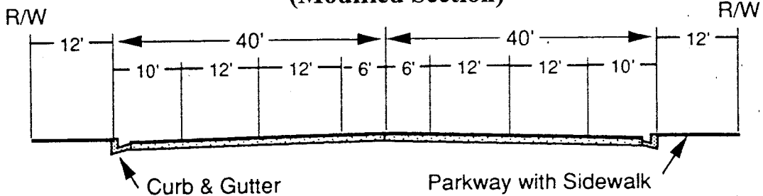
Major Highway 104' Right-of-Way
