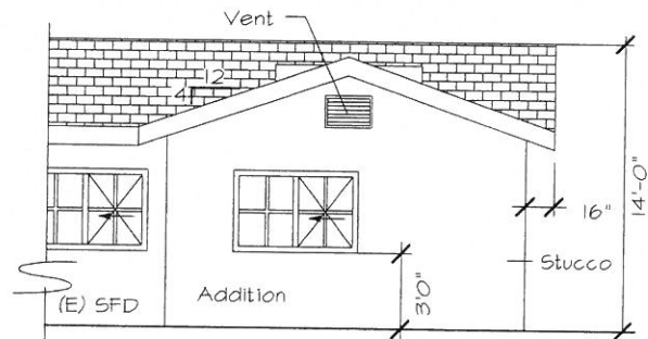
NORTH ELEVATION
