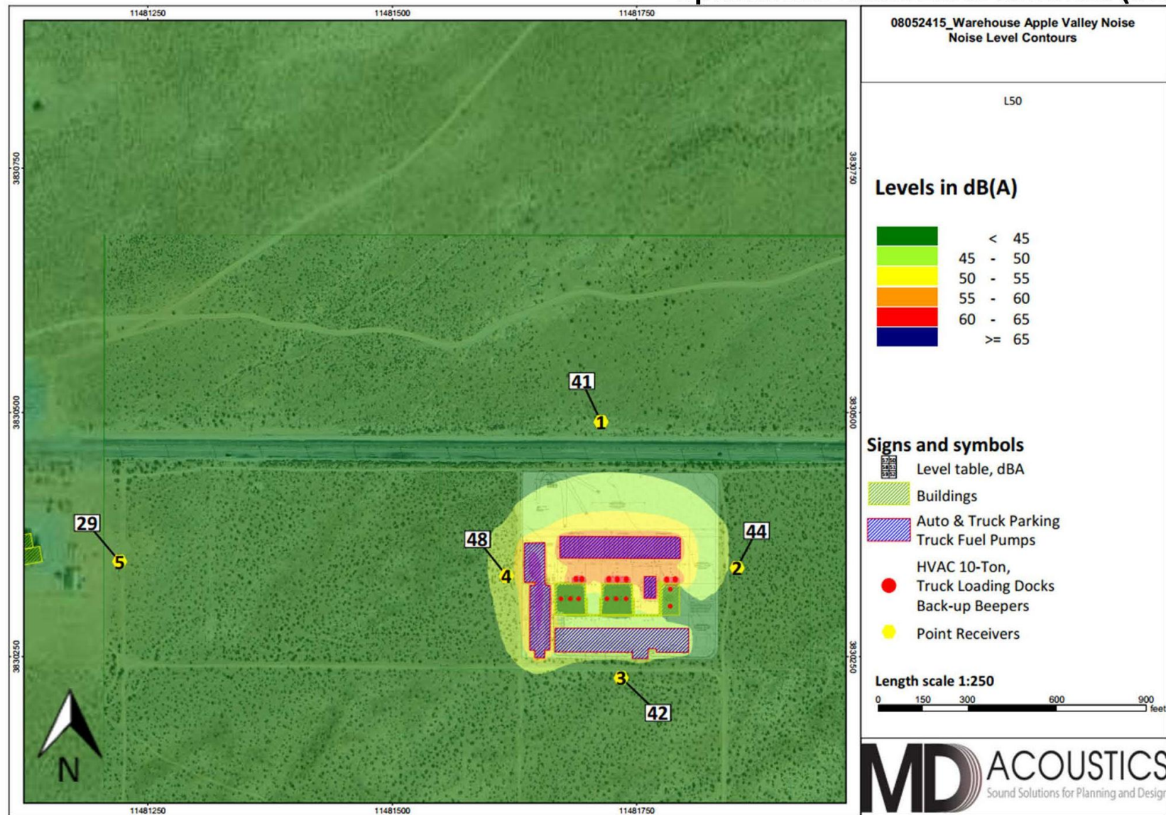
Figure 8: Operational Noise Contours
