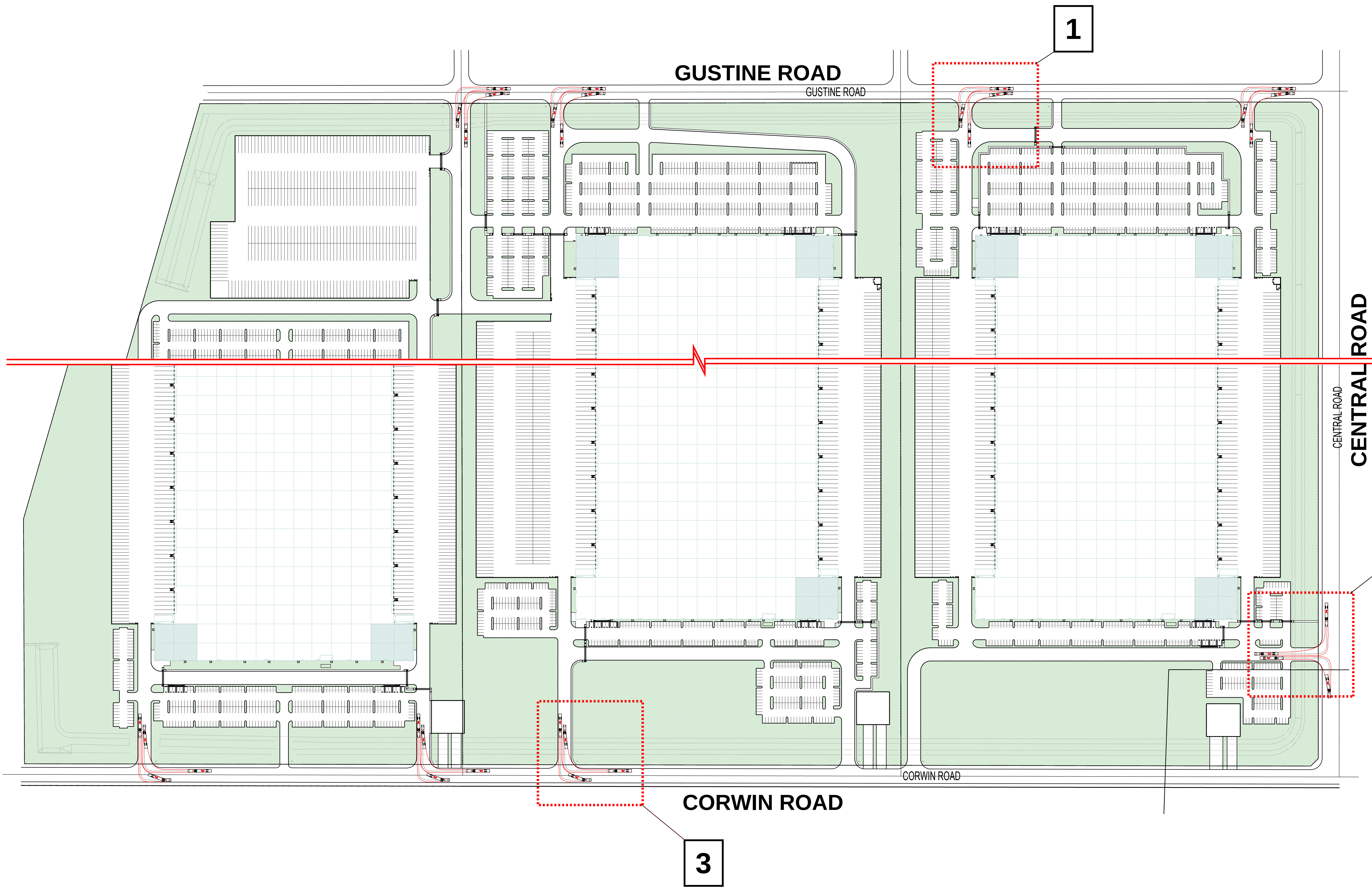
1 TYP. TRUCK TURN AT GUSTIN ROAD
