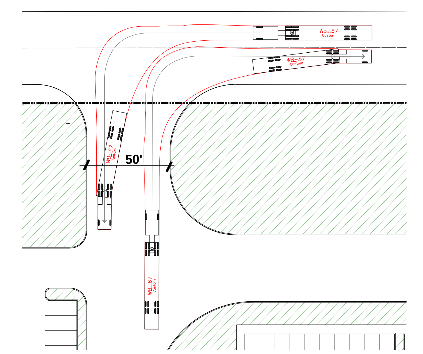
1 TYP. TRUCK TURN AT GUSTIN ROAD
