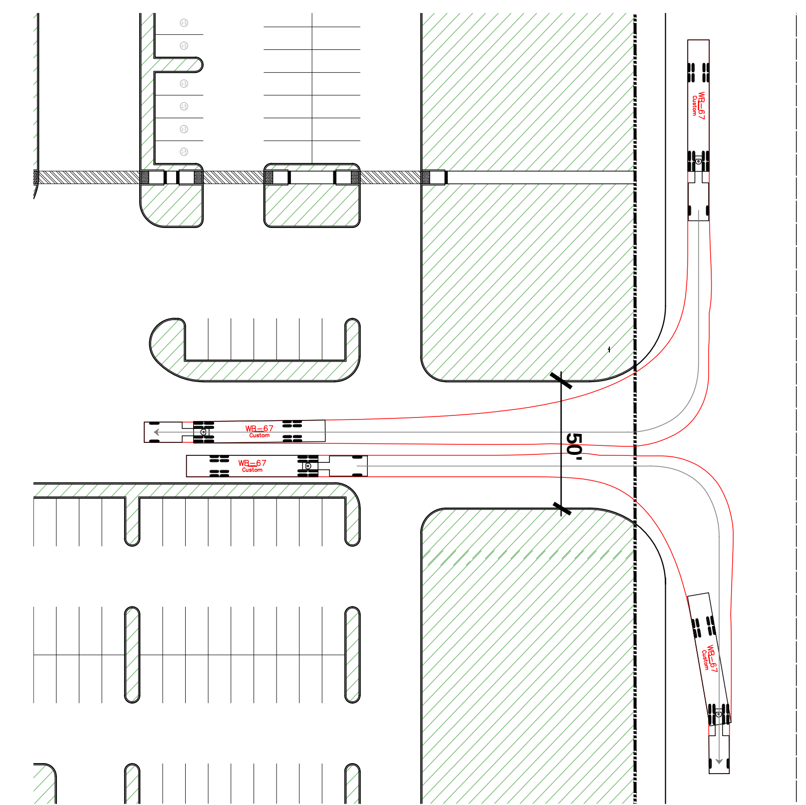
1 TYP. TRUCK TURN AT GUSTIN ROAD
