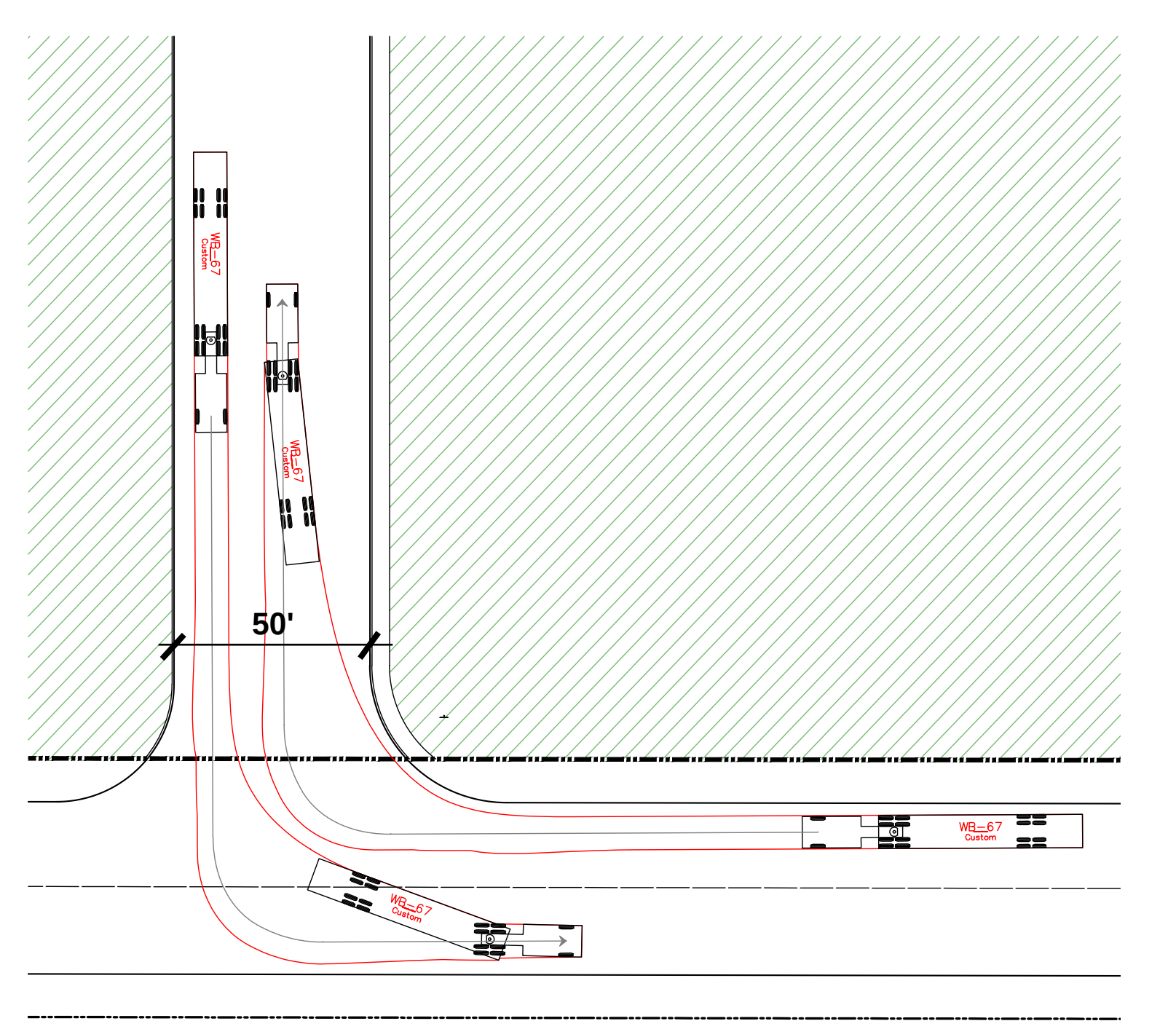
2 TRUCK TURN AT CENTRAL ROAD
